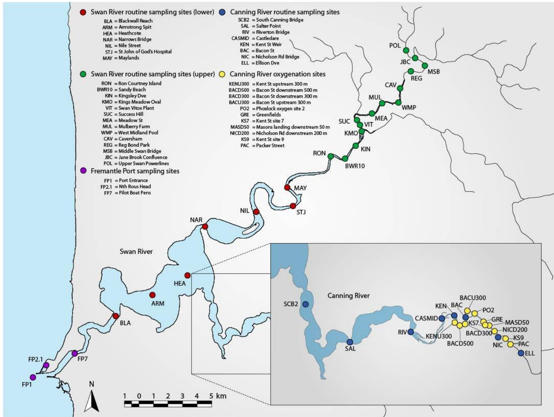
Figure 1: Map showing routine Swan Canning Estuary sampling sites
